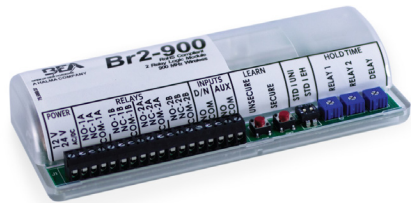
BR2-900 2-Relay Logic Module + 900 MHz Wireless Technology
